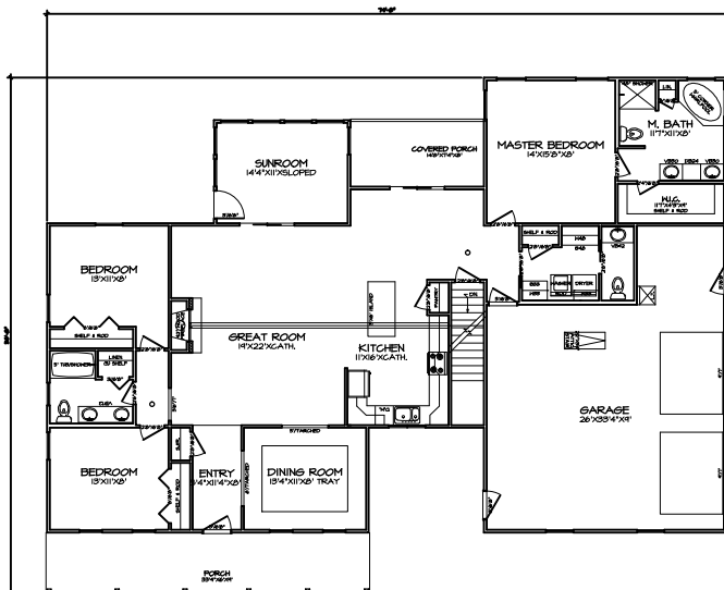
1 FIRST FLOOR PLAN A-3
