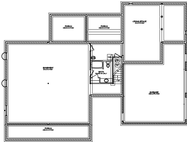
1 FOUNDATION PLAN A-2
